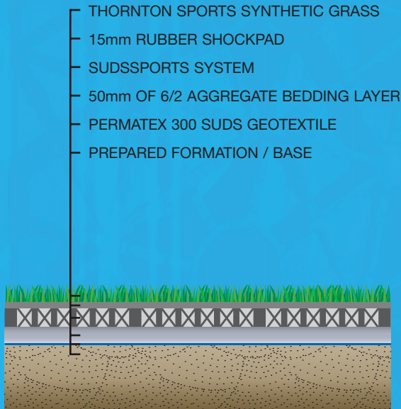
TYPICAL SUDSPORTS PITCH CROSS SECTION
